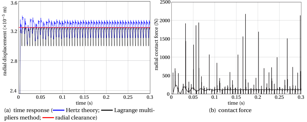
FIGURE 5: Responses through Lagrange multipliers method at \omega = 50 Hz and \gamma_0 = 30 \mu\text{m}
