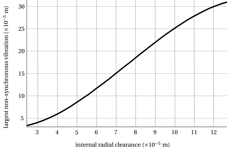
FIGURE 9: Largest non-synchronous vibration with respect to IRC ( m e = 4 \times 10^{-5} m and N_b = 8 )
