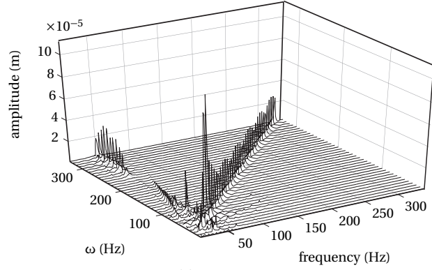
(a) \gamma_0 = 20 \mu\text{m}
