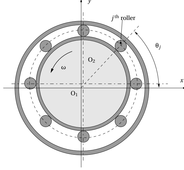
FIGURE 3: Bearing Contact Model
