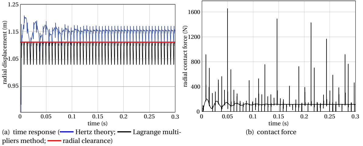
FIGURE 4: Responses through Lagrange multipliers method at \omega = 50 Hz and \gamma_0 = 10 \mu\text{m}
