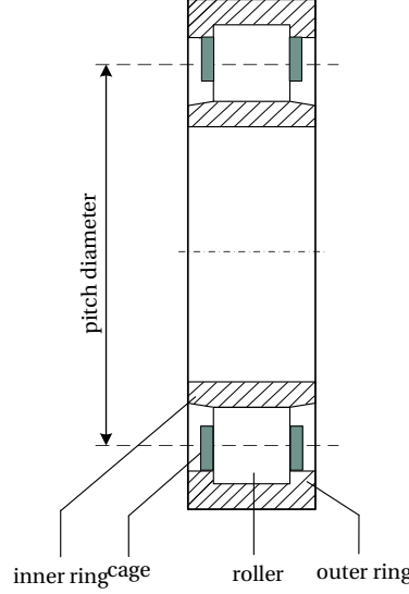
FIGURE 2: Roller bearing of interest
