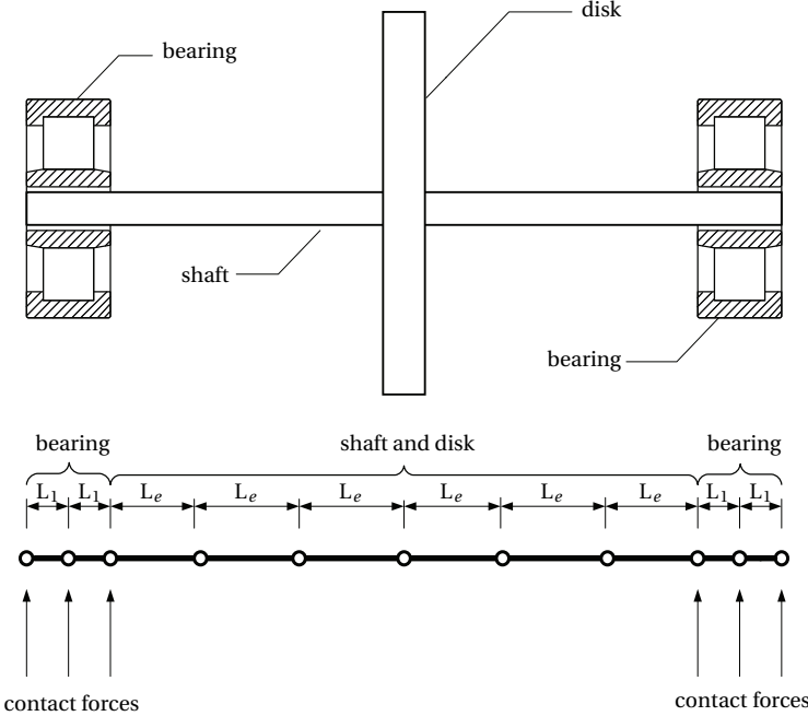
FIGURE 1: Finite element model of the rotor bearing system
