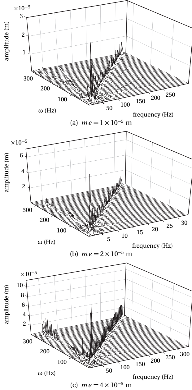
FIGURE 7: cascade diagram under effects of the mass imbalance ( N_b = 8 and \gamma_0 = 20 \mu\text{m} )
