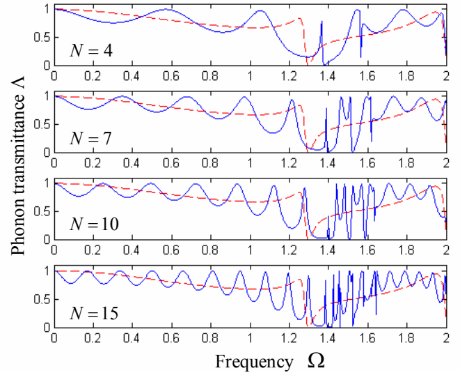
Figure 6: Phonon transmittance vs. scattering frequency for staircase having a variable number N of steps in the case of stiffened force constants in the perturbed step region. The dotted line refers to single step for the same parameters.
