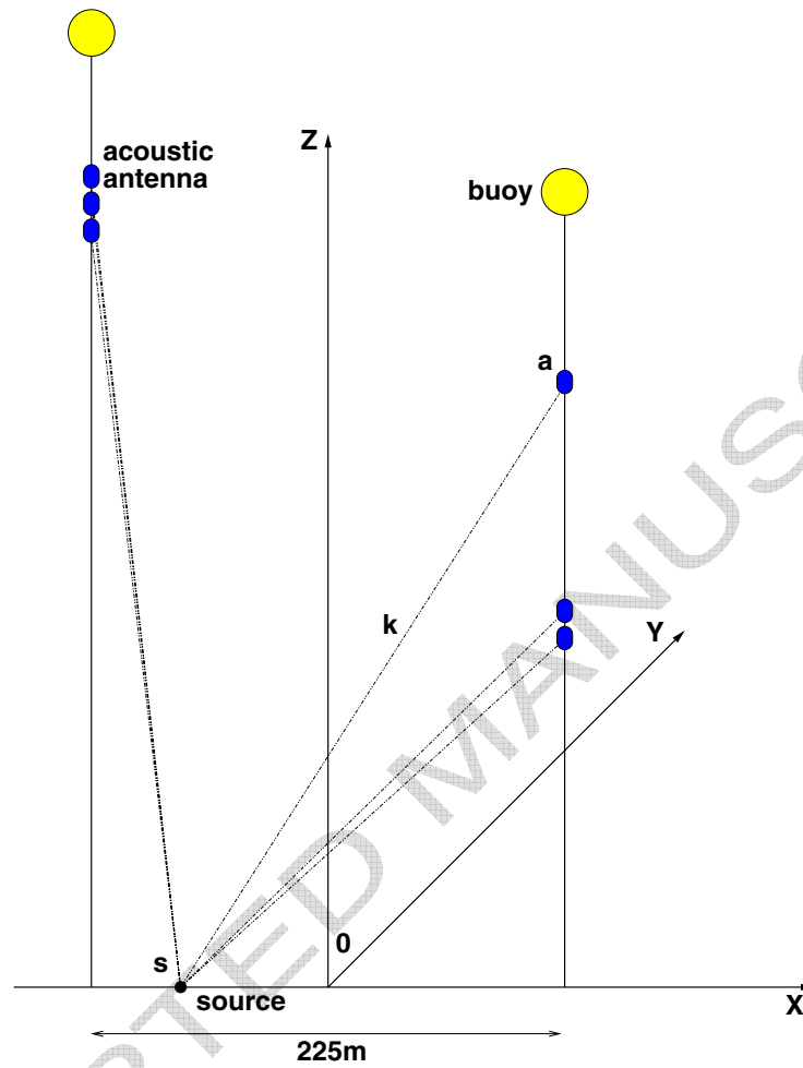
Fig. 10. The geometry of the simulated acoustic setup. The lines are 225 m apart, the vertical position of the stories are 180 m , 195 m and 305 m for the line on the right and 390 m, 405 m and 420 m for the line on the left.
