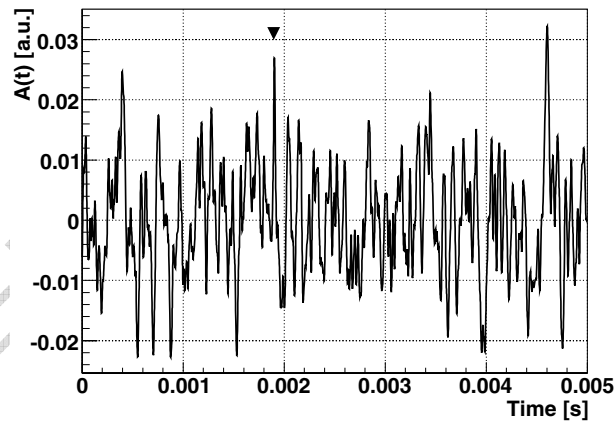
Fig. 5. After application of a cross correlation the lower frequencies are removed. The signal to noise ratio is improved. The marker indicates the signal position.
