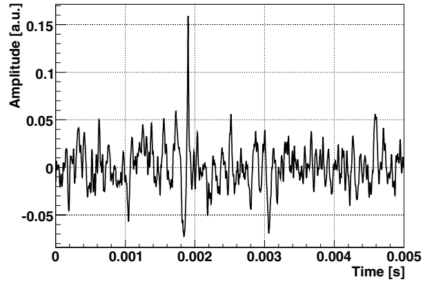
Fig. 6. Stacked output of six hydrophones. The signal at 0.0019 s becomes clearly visible.
