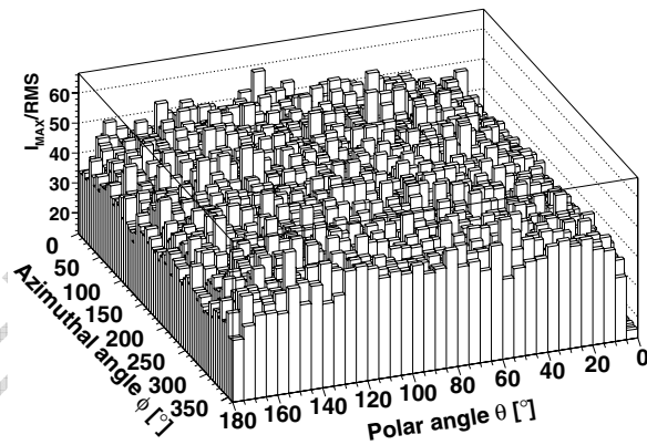
Fig. 9. Maximum pressure amplitude from the beamforming algorithm divided by the RMS of the data, for all directions.
