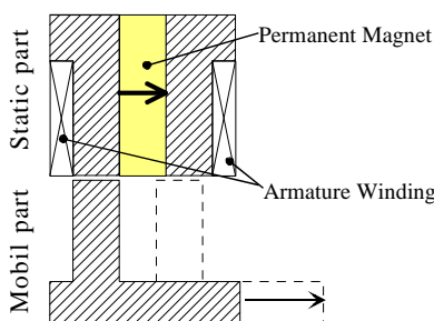
Fig.1. Elementary cell of the machine
