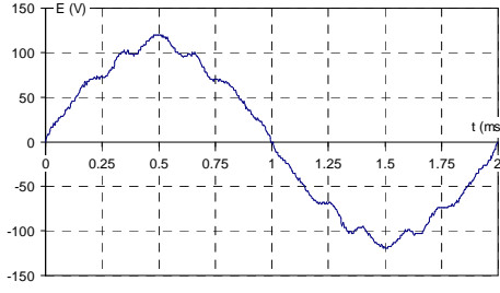
Fig.4.Measured EMF at 3,000 rpm
