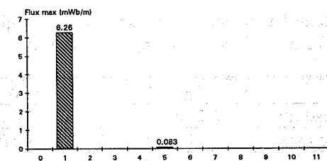
Fig. 11. Frequency spectrum of the no-load flux
