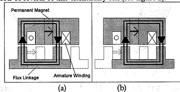
Fig. 1. The two conjunction positions
