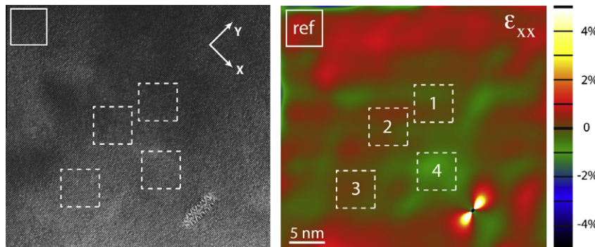
Fig. 1. Example of the determination of the mean value and standard deviation of strain \epsilon_{xx} for the lath-shaped precipitate in Fig. 3. The values in the different areas are reported in Table 1. “Ref.” corresponds to the area taken as the strain-free reference.
