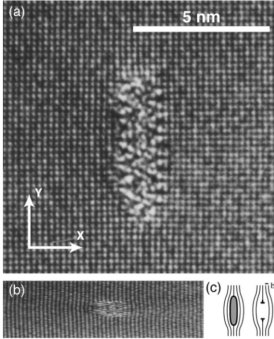
Fig. 3. Lath-shaped precipitate in the Al-6056-T6 alloy: (a) HRTEM image; the electron beam is the [0\ 0\ 1] direction of the Al matrix; (b) part of the same image but shrunk in the vertical direction to exemplify the distortion of the matrix parallel to the horizontal axis; (c) schematic of the horizontal displacements around a lath-shaped precipitate and around a dipole of edge dislocations.
