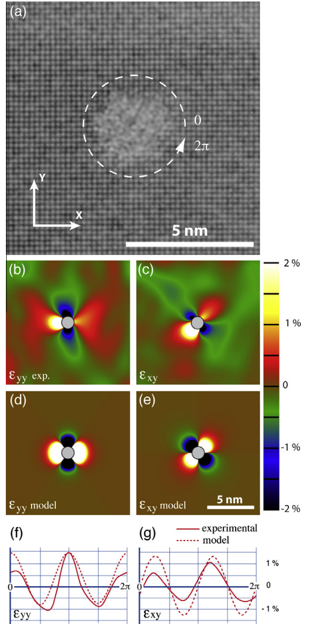
Fig. 2. Rod-shaped precipitate in the Al-6056-T6 alloy: (a) HRTEM image; the electron beam is the [001] direction of the Al matrix; (b) and (c) experimental strain \varepsilon_{yy} and \varepsilon_{xy} ; (d) and (e) modeled \varepsilon_{yy} and \varepsilon_{xy} strain fields corresponding to an Eshelby inclusion with infinite size in the [001] viewing direction and a radial displacement field u_r = -0.08r^{-2} fitted by comparing the experimental and modeled displacement fields; (f) and (g) line profiles of (d) and (e) at a constant distance (2 nm) from the symmetry center of the rod (along the dotted line in (a)).
