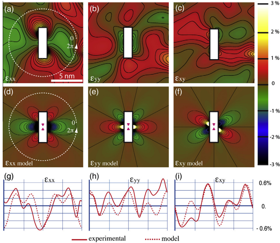
Fig. 5. Experimental and modeled strain fields around the lath-shaped nano-particle in Fig. 4: (a) \epsilon_{xx} ; (b) \epsilon_{yy} ; (c) \epsilon_{xy} ; (d)–(f) represent the modeled strain fields around a dipole of edge dislocations (iso-values every 0.2%); (g) and (h) the line profiles made at a constant distance (5.4 nm) from the symmetry center of the precipitate (along the dotted line in (a)).
