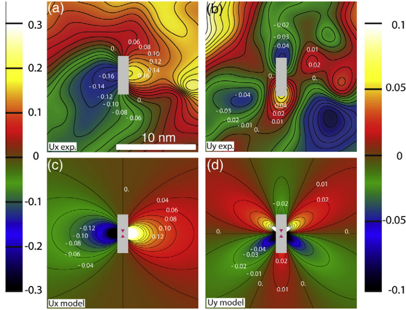
Fig. 4. Displacement fields around the lath in Fig. 3: (a) experimental displacements u_x in the horizontal direction; (b) u_y in the vertical direction; (c) and (d) the corresponding modeled fields components. For the measured and modeled displacement fields, u_x presents a diad symmetry (vertical mirror plane), while u_y shows a pseudo three-fold symmetry (vertical mirror plane and at \pm 120^\circ ).
