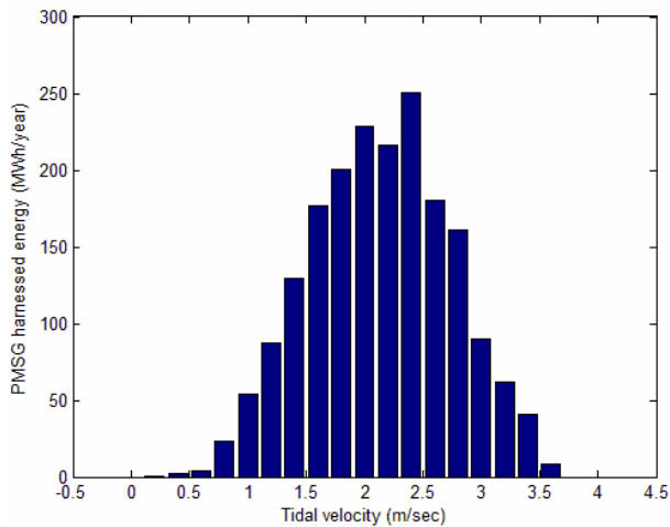
Fig. 15. PMSG-based MCT harvested energy histogram in one year.
