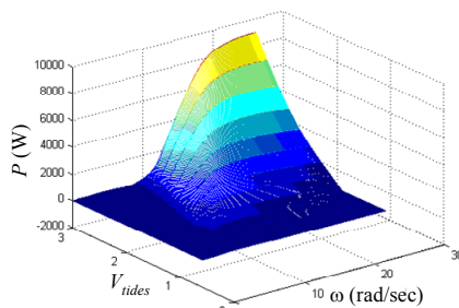
(b) The extractable power P(\omega, V_{tides}) .
