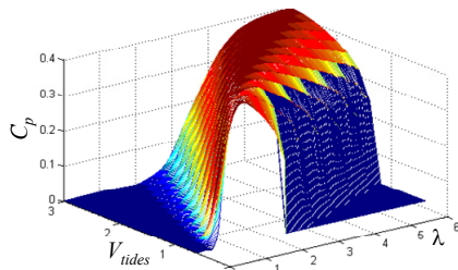
(a) C_p(\lambda, V_{tides}) curves.
