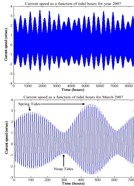
Fig. 4. Tidal velocity in the Raz de Sein for the year 2007 and March 2007.
