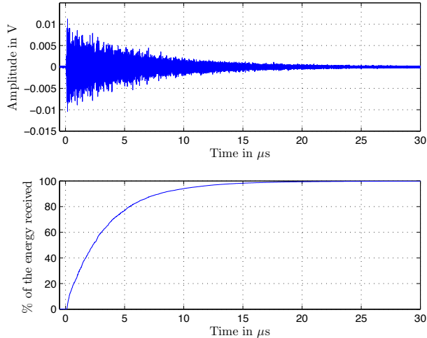
Fig. 5. Measured channel impulse response in the empty RC and percentage of the total energy of the impulse response vs. time
