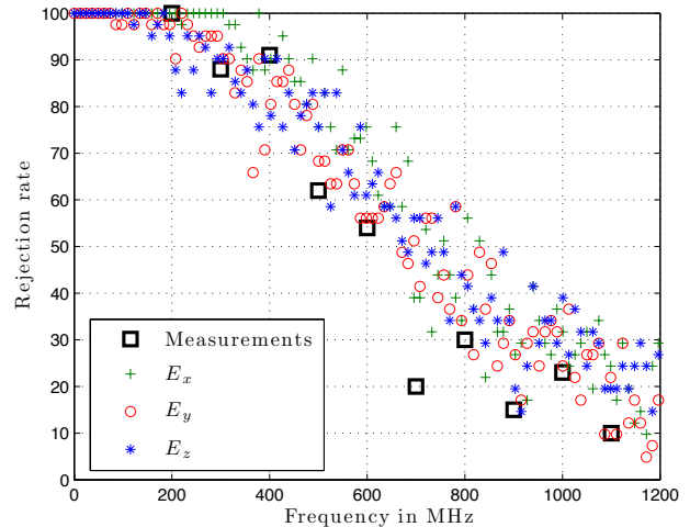
Fig. 7. Rejection rate in % with AD GoF test for the Rayleigh distribution with N = 100 vs. frequency. Results from E-field measurements and from simulations with R = 0.998 .
