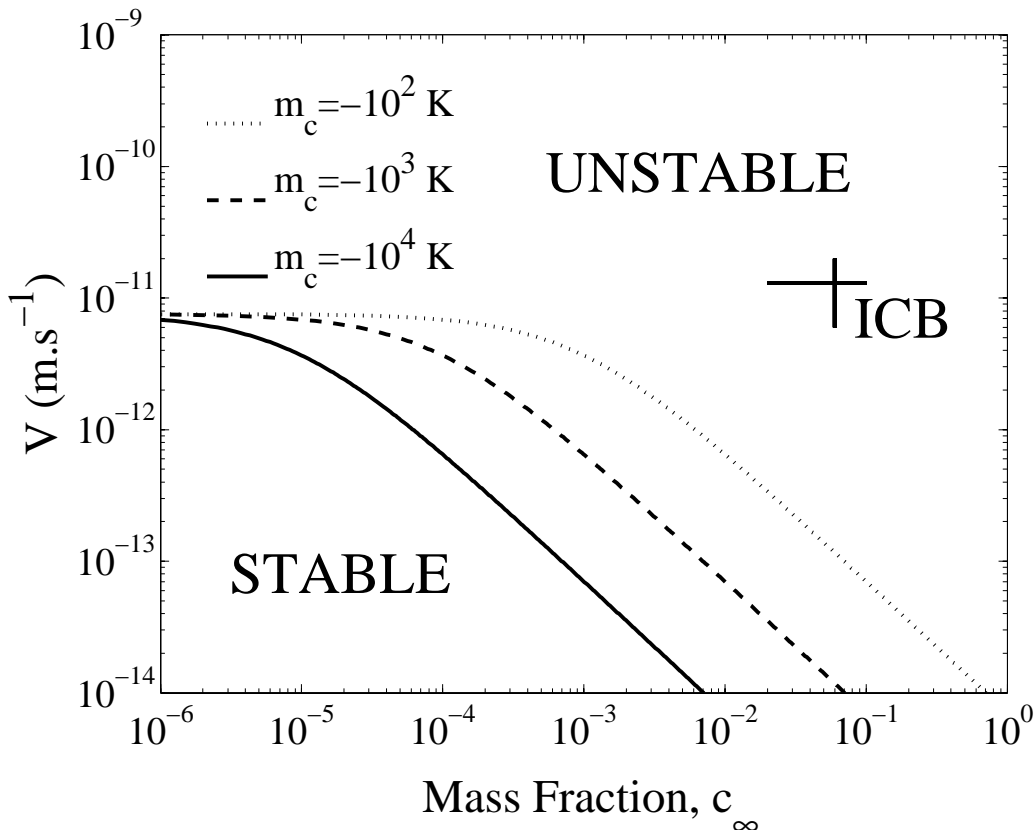
Fig. 3. Neutral curves for linear morphological stability, with m_c = -10^2 K (dotted line), m_c = -10^3 K (dashed line) and m_c = -10^4 K (solid line). G_T^s = 0 K.m ^{-1} and k = 0.25 . The straight lines cross is the location of the ICB in the stability diagram. Uncertainties in V result from uncertainties in the age of the inner core. The value of c_\infty depends on the chemical model chosen: c_\infty \simeq 10 wt.% if there is only one dominant light element, and c_\infty \simeq 2 wt.% if the model of Alfe et al. (2002) is adopted.
