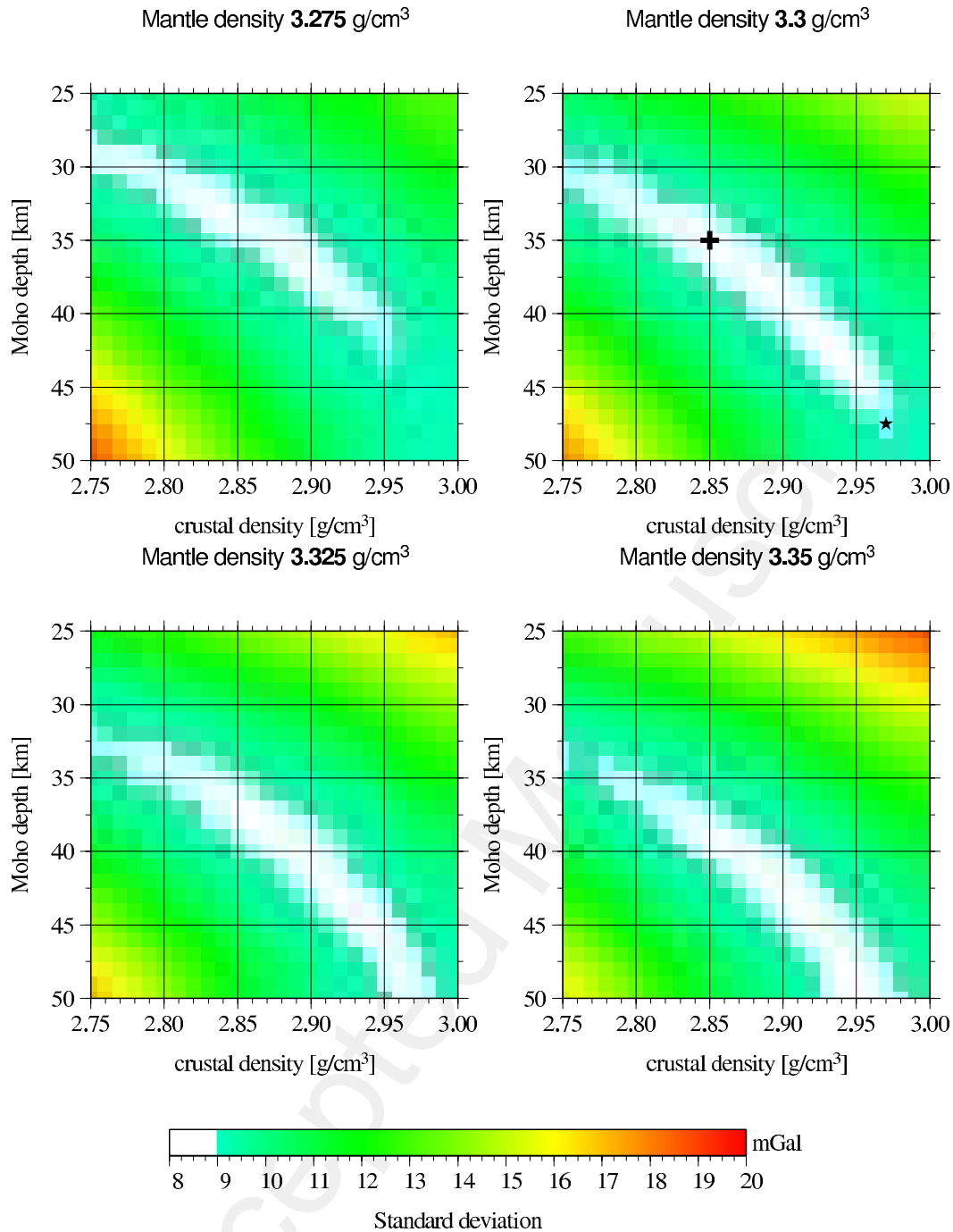
Figure 8. Results of grid search for densities and Moho depth below western Crete. Symbols indicate parameters of Model I (+: \rho = 2850 \text{ kg/m}^3 , \text{depth} = 35 \text{ km} ) and Model II (★: \rho = 2970 \text{ kg/m}^3 , \text{depth} = 47.5 \text{ km} ).
