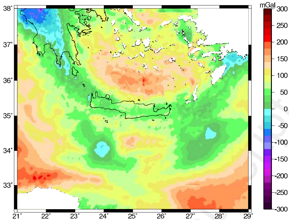
Figure 3. Bouguer gravity field \rho_B = 2670 \text{ kg/m}^3 of the Hellenic subduction zone.
