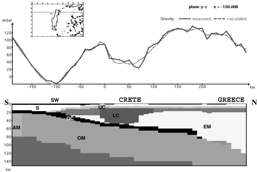
Figure 9. SN cross-section of the density model through western Crete (Model II). Upper part - anomalies, lower part - density structure.
