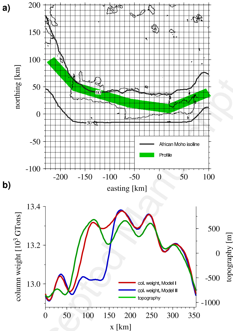
Figure 10. a) Profile of mass distribution analysis b) topography with calculated weight of columns along the profile.
