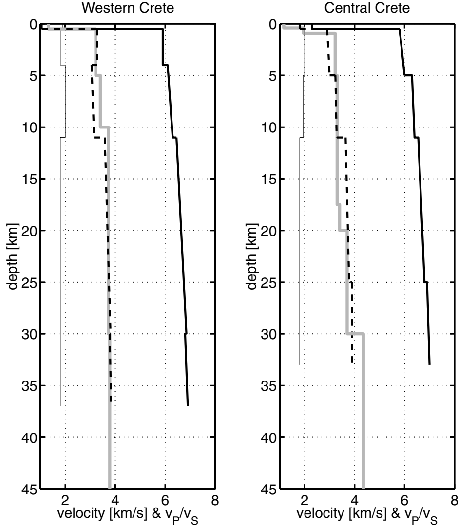
Figure 2. Seismic constraints on elastic parameters beneath western and central Crete. Black lines denote parameter values from seismic profile lines, i.e. P-wave velocity (thick solid line), S-wave velocity (thick dashed line) and v_P/v_S ratio (thin solid line). Thick grey lines indicate S-wave velocity models from surface wave dispersion modelling.
