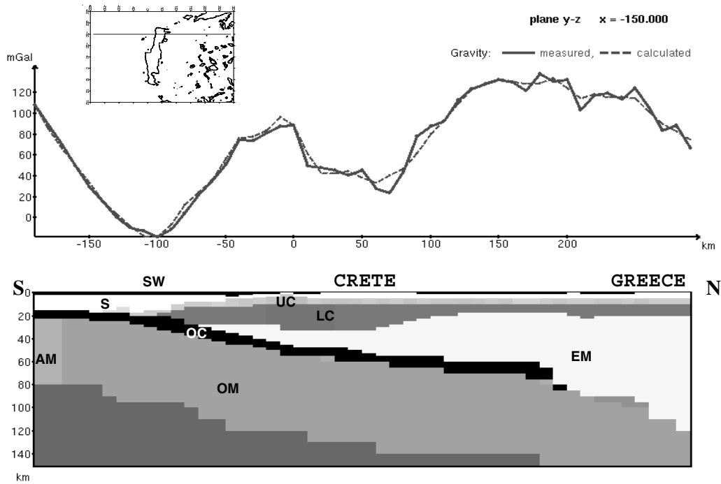
Figure 5. SN cross-section of the density model through western Crete (Model I). Upper part - anomalies, lower part - density structure.
