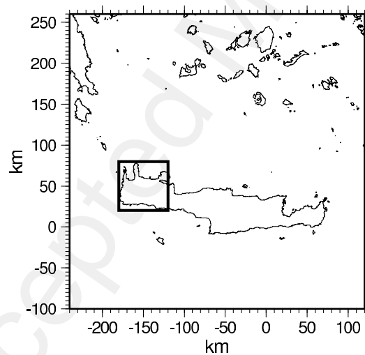
Figure 7. Area defining part of model chosen for grid search analysis.
