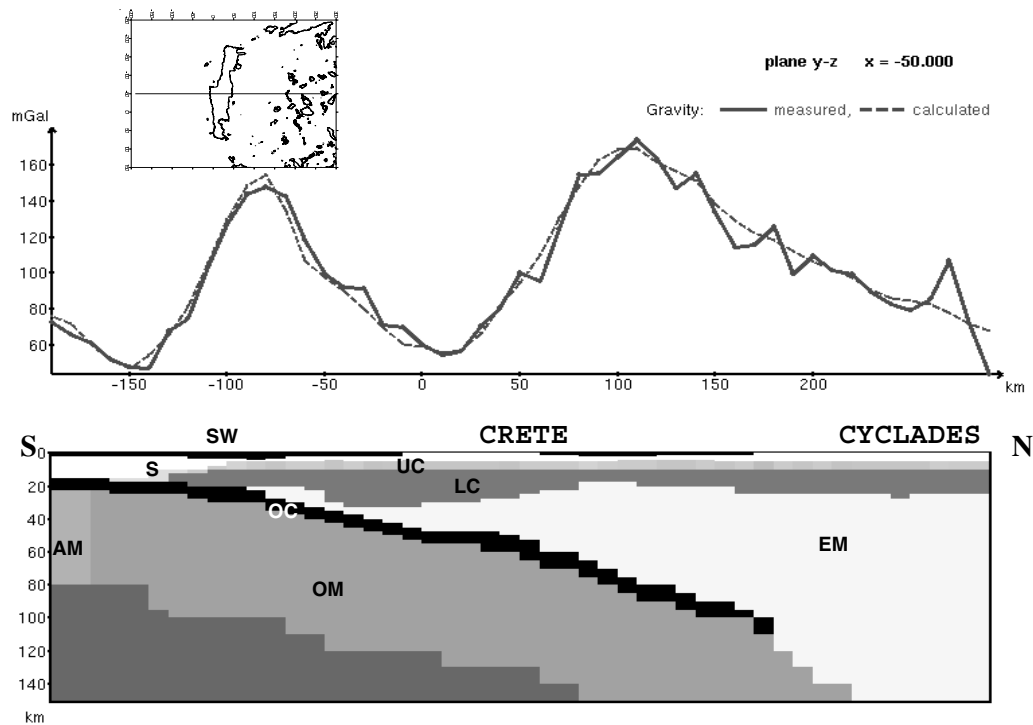
Figure 6. SN cross-section of the density model through central Crete (model I). Upper part - anomalies, lower part - density structure.
