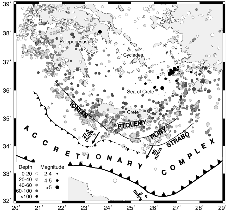
Figure 1. Map of the Aegean region showing major tectonic units and earthquake hypocenters from the relocated ISC catalogue (Engdahl et al., 1998) for 1964 to 1998. The southern deformation front of the Hellenic subduction zone and the border between the central and inner units of the Mediterranean ridge (Lallemant et al., 1994; Huguenot et al., 2001) are indicated. Horizontal GPS velocities relative to Eurasia (McClusky et al., 2000) are depicted by arrows. Additionally, trenches south of Crete are delineated.
