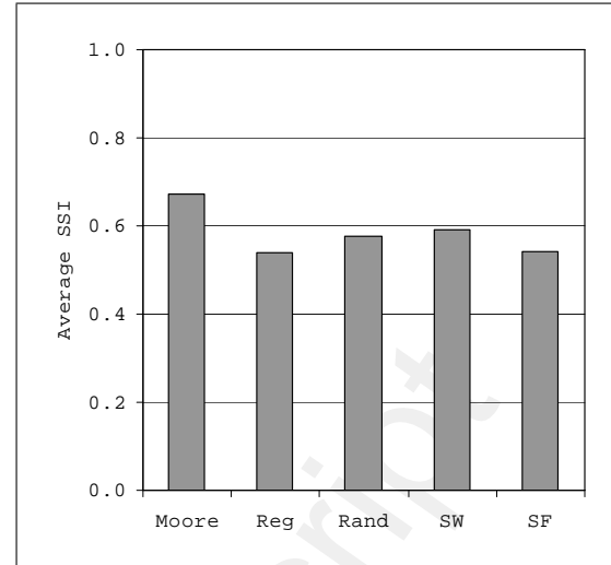
Figure 9: Average Spectral Segregation Index (SSI) v. Network Classes. Average Degree d = 8 . Parameters: M = 100 , \theta = 0.3 . MC Sample Size = 1000.
