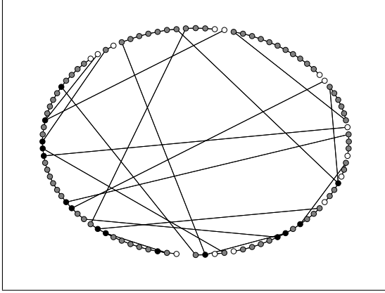
Figure 4: An example of a small-world graph obtained from M = 100 nodes originally lying on a circle and interacting with their nearest neighbors only ( r = 1 ). Rewiring probability \beta = 0.2 . Nodes color depends on degree after rewiring. Black nodes: d \geq 3 . Grey nodes: d = 2 . White nodes: d = 1 .
