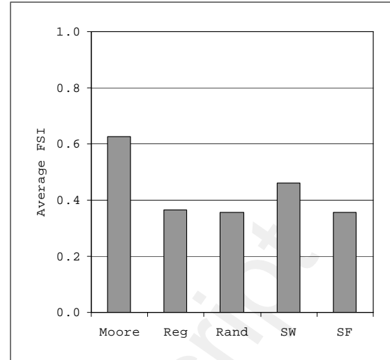
Figure 7: Average Freeman’s Segregation Index (FSI) v. Network Classes. Average Degree d = 8 . Parameters: M = 100 , \theta = 0.3 . MC Sample Size = 1000.
