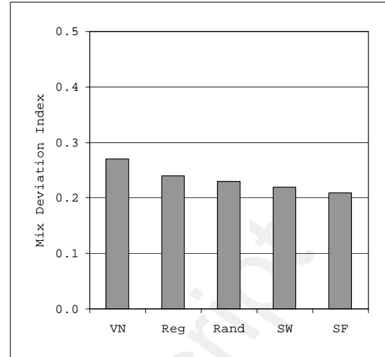
Figure 13: Average Mix Deviation Index v. Network Classes. Average Degree d = 4 . Parameters: M = 100 , \theta = 0.2 . MC Sample Size = 1000.
