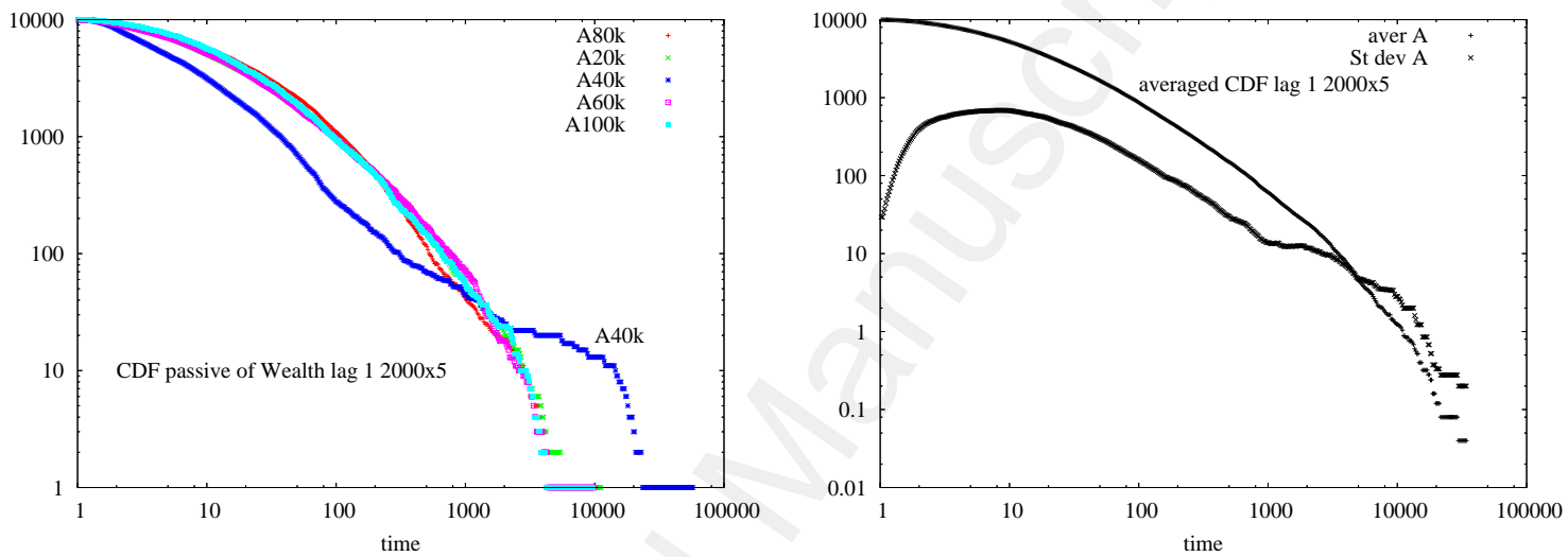
Figure 9: Cumulative distributions of wealth in the absence of avalanches, after several ten thousands iteration steps. The left diagram is a series of histograms at different times: even after long evolution, the distribution may still fluctuate by large amounts. The right diagram shows the time-averaged distribution of net worth and standard deviation of net worth. Parameter setting is the same as for the previous figures.
