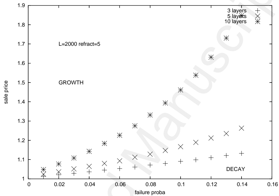
Figure 4: Regime diagram in the sale price versus probability of failure plane. The time lag between bankruptcy and re-birth is 5. The two regions of growth and economical collapse at large times are separated by lines whose position are fixed by simulation parameters. We here varied the production network depth: the '+' line was obtained for a 3 layers net, the 'x' line for a 5 layers net, and the '*' line for a 10 layers net.
