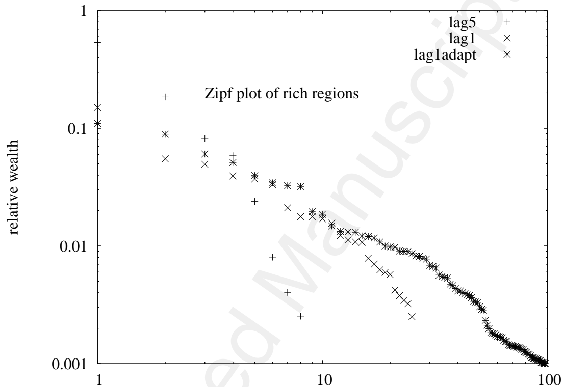
Figure 8: Zipf plot of wealth of the most active regions for the standard and adaptive firms models (cf. section 4.1). The vertical axis displays the production relative to the total production. The '+' signs correspond to the standard model with time lag = 5, the 'x' to time lag = 1, and the '*' to the adaptive firms model with time lag = 1.
