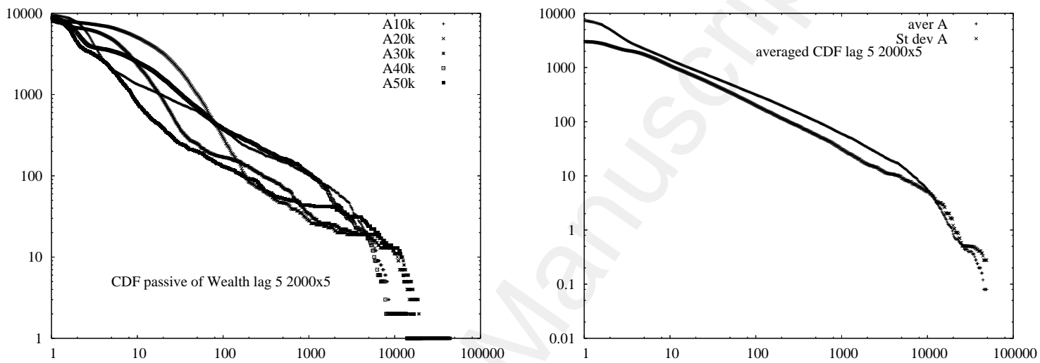
Figure 10: Cumulative distributions of wealth in the avalanche regime (the time lag is 5) after several ten thousands iteration steps(left diagrams). Even after such long evolutions, the distribution fluctuates by large amounts. The right diagram shows the time-averaged distribution of net worth and standard deviation of net worth. Parameter setting is the same as for the previous figures.
