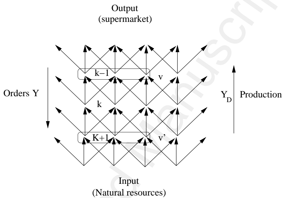
Figure 1: Firms are located at the nodes of the lattice. Production ( Y^D ) flows from the resource input layer ( k = l ) to the output layer ( k = 0 ); orders ( Y ) flow backward. The v and v' are respectively the output and input neighborhoods of a firm at level k .
