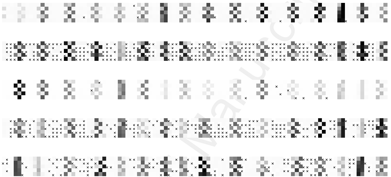
Figure 11: Series of wealth and patterns for a network of "adaptive" firms. The conventions and parameters are the same as for figures 5 and 6, for a 100 \times 5 lattice. Time lag is 1. Patterns are taken at time 2000 (for the lower pattern) and 4000, 6000, 8000, 1000 upward. The position of the rich regions are stable, but their relative amplitude varies.
