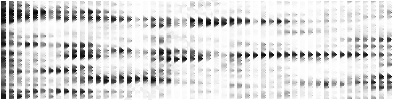
Figure 7: Successive patterns of wealth from left (at time 200) to right (at time 10000). These patterns are rotated by 90 degrees with respect their orientation in figures 5 and 6. Input layer is the left layer of each pattern. Following the horizontal axis we see that patterns are metastable, with life times of the order of a few thousands (parameter set-up: time lag = 1, 100x5 lattice).
