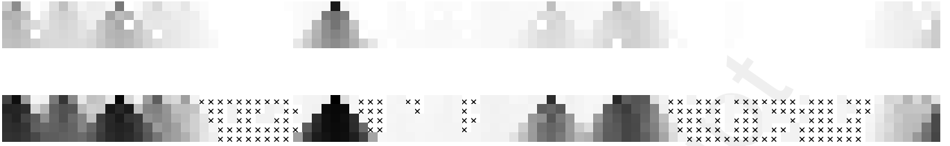
Figure 6: Patterns of wealth(upper pattern) and production (lower pattern) after 2500 iterations steps with the parameter set-up of figure 3 (right) (time lag is 5). The same alternance of active and less active regions is observed, but with a larger time lag (5), we also get large zones of bankrupted firms signaled by crosses (x).
