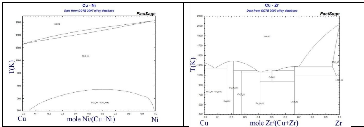
Figure 1 : Binary phase diagrams, Cu-Ni (a), Cu-Zr (b) from [13]
