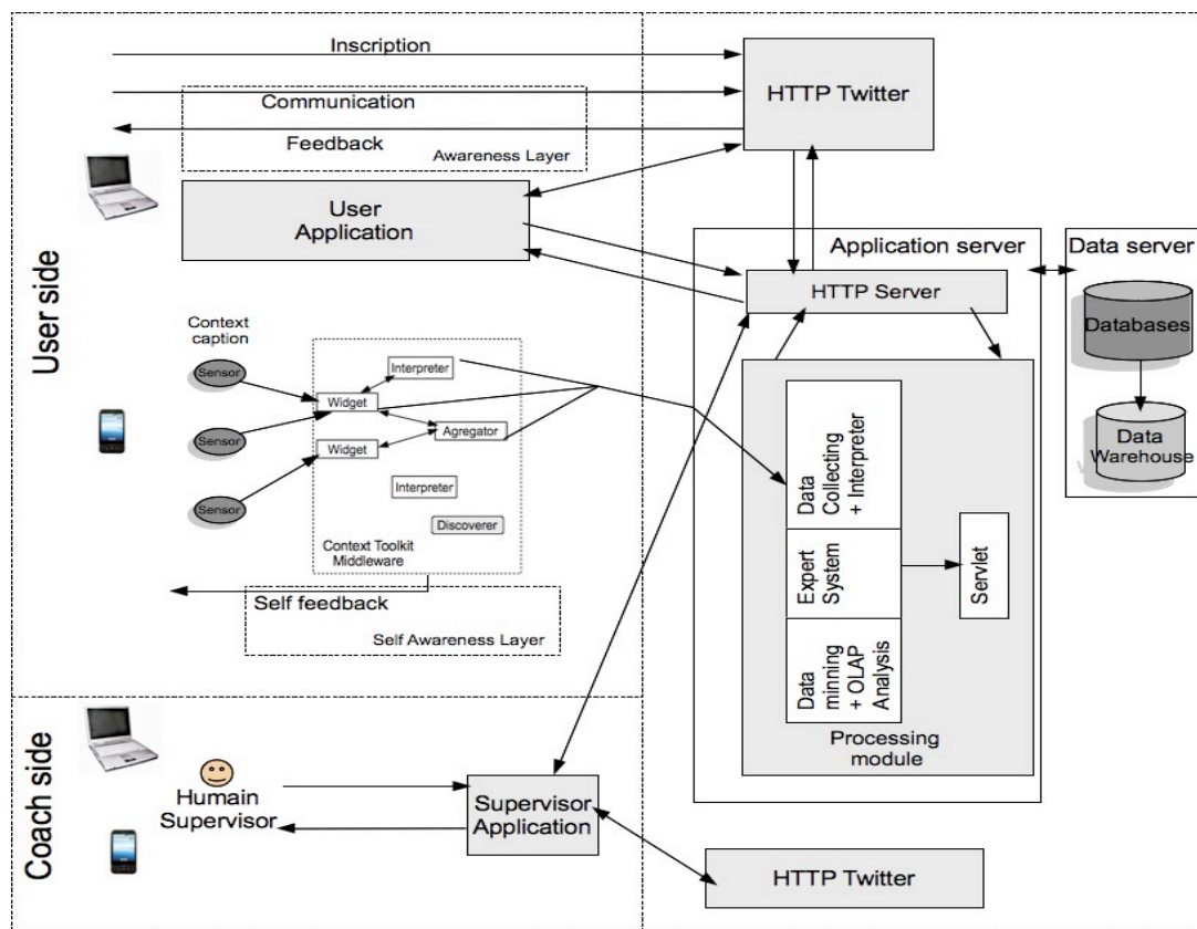
Figure1. TwittGym architecture
