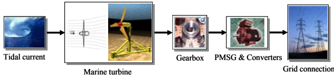
Fig. 1. Marine current turbine global block diagram.
