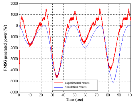
Fig. 16. Output power: Experimental vs simulation.
