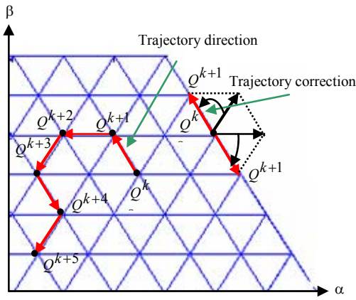
Fig. 7. Optimal space vector tracking and trajectory correction in the stationary \alpha\beta frame.
