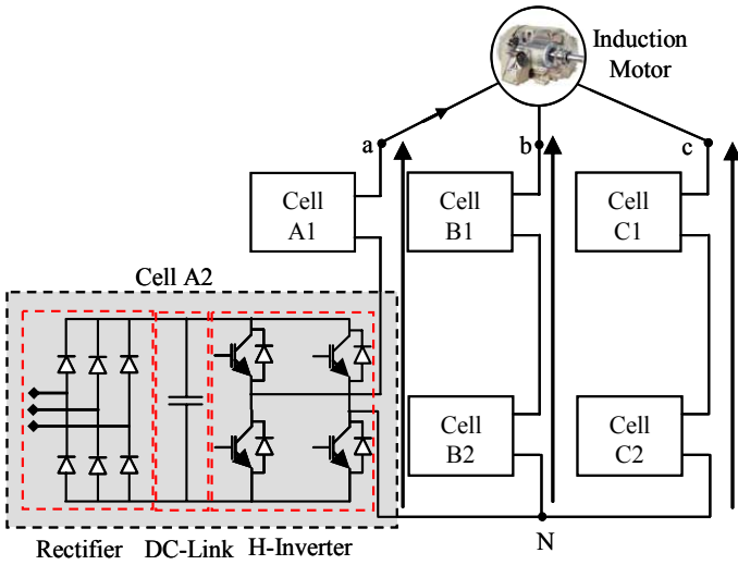
Fig. 1. Asymmetric cascaded H-bridge multilevel inverter.
