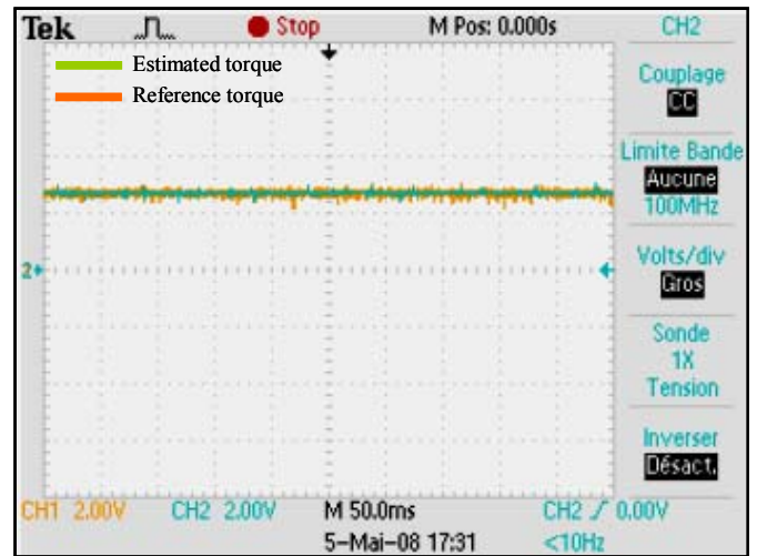
(a) Reference and estimated torque waveforms.
