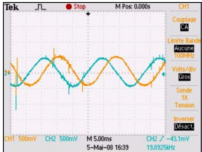
(b) \alpha - \beta flux component waveforms.
