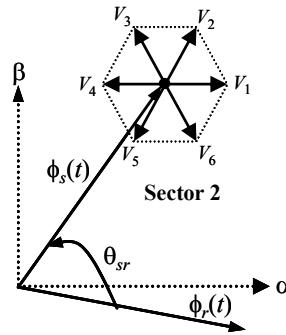
Fig. 6. Voltage selection \Delta v_s^k in sector 2.
