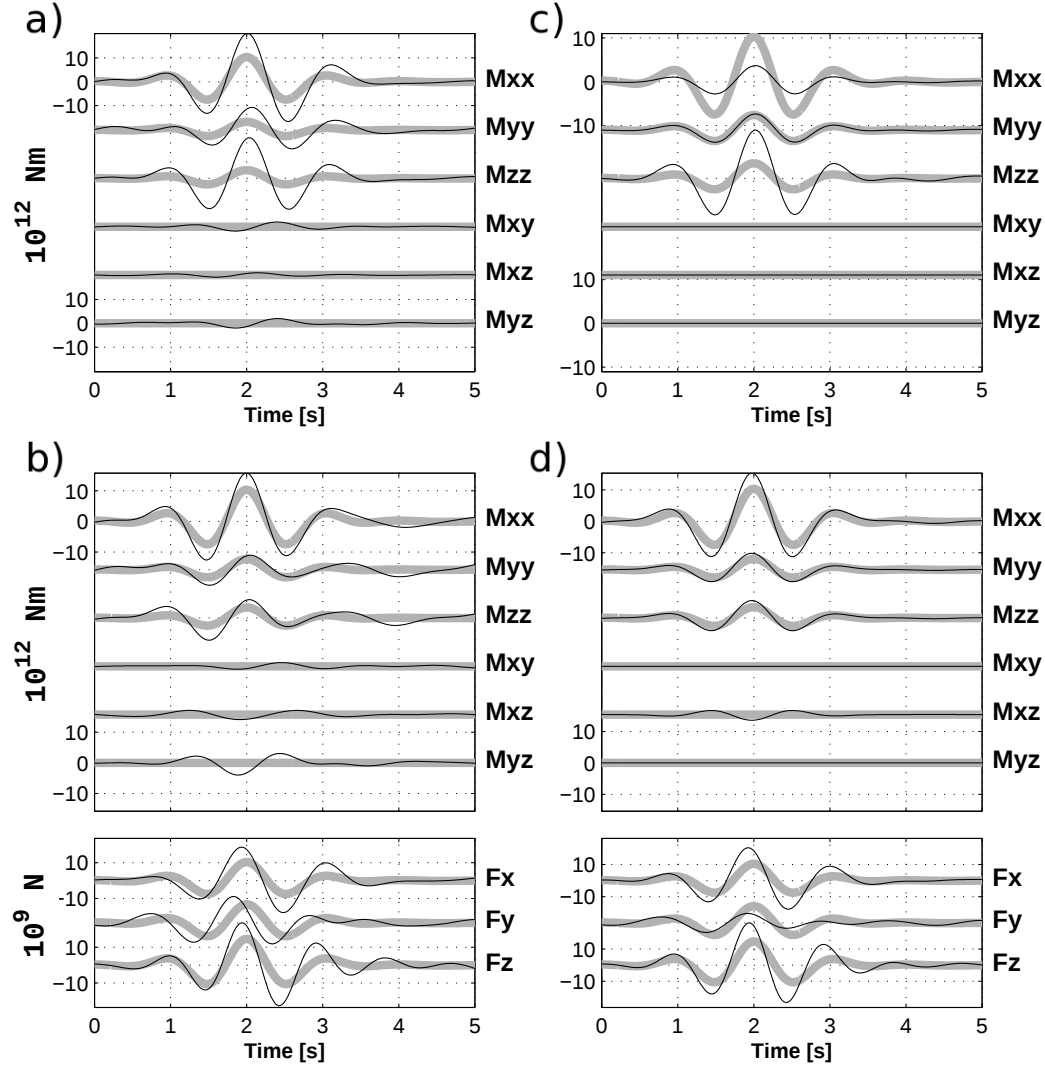
Figure 5. Source Time Function (black thin lines) reconstructed using a) unconstrained inversion for moment only (MT), b) unconstrained inversion for moment and single forces (MT+F), c) constrained inversion for crack only (Cr), d) constrained inversion for crack and single forces (Cr+F). Noisy synthetic data are computed for the vertical crack C_X and inclined single force F_{45} , whose source mechanism is shown by the thick grey lines. In the figure, amplitude is 10^{12} N.m for the moment and 10^9 N for the single forces.
