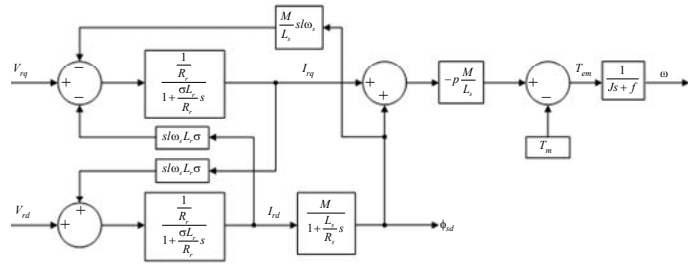
Fig. 6. Overall block scheme for DFIG variable speed control.
