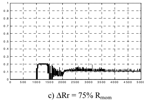
Fig. 3. Fuzzy output of the detection block (FS).
