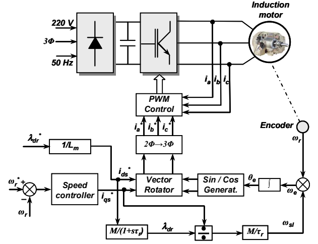
Fig. 1. Direct field-oriented induction motor drive.
