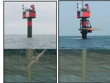
Fig. 7. Hybrid illustration of the Seaflow turbine [© MCT].
