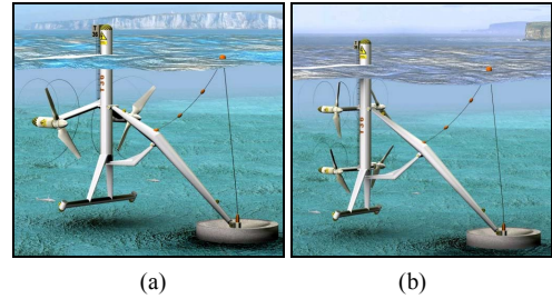
(a) (b) Fig. 10. The Tidal Stream concept [© Tidal Stream].
