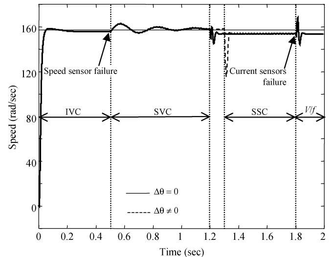
Fig. 14. Speed response according to controller transitions.
