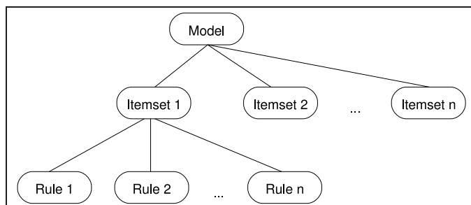
Fig. 5 The content of an association model in Microsoft SQL server 2005.
