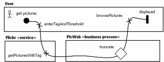
Figure 1: AoUCM: Root Map – Get Pictures
