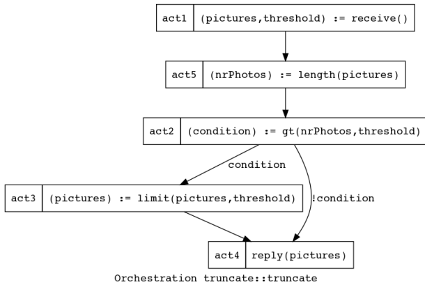
Figure 7: ADORE: truncate Business Process
