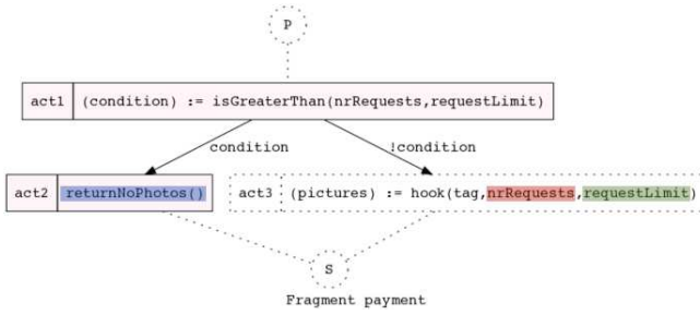
(a) Generated Design Artifact (with design weaknesses)
