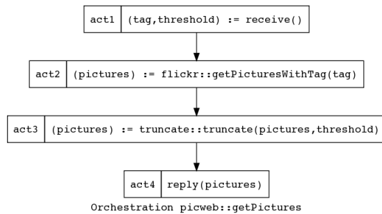
Figure 6: ADORE: getPicture Business Process
