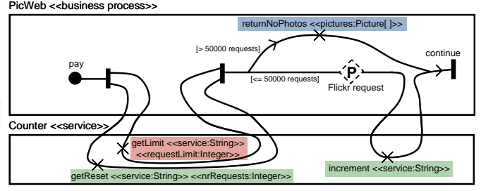
(b) Enhanced Requirements Artifact (weaknesses addressed)
