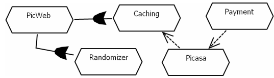
Figure 4: Concern Interaction Graph
