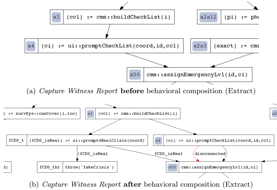
Fig. 5. Illustrating the fragment weave process on Capture Witness Report
