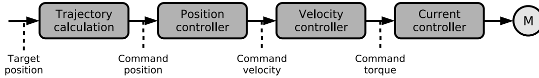
Figure 4: The internal flow control between the individual controllers inside the drive control unit. Depending on the type of the command value, different controllers are active. The control loops are closed by the feedback of the rotary encoder on the motor, and a possible controller on the load axis, as well as the measurement of the current.
