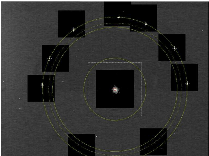
Figure 8: A measurement of a star for the calibration of the pointing model. Visible are the seven LEDs and their determined center of gravity, as well as the reconstructed circle on which the LEDs are located. The LEDs on the bottom part are hidden by the lower lid, holding a screen in front of the camera. The black regions are the search regions for the LEDs and the calibration star. A few dead pixels in the CCD camera can also be recognized.
