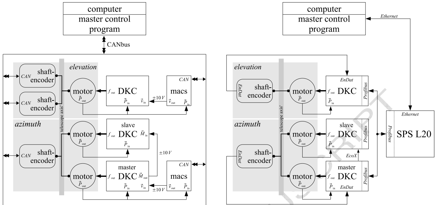
Figure 2: Schematics of the MAGIC I (left) and MAGIC II (right) drive system. The sketches show the motors, the motor-encoder feedback as well as the shaft-encoder feedback, and the motion-control units, which are themselves controlled by a superior control, receiving commands from the control PC, which closes the position-control loop. The system is described in more details in section 4.
