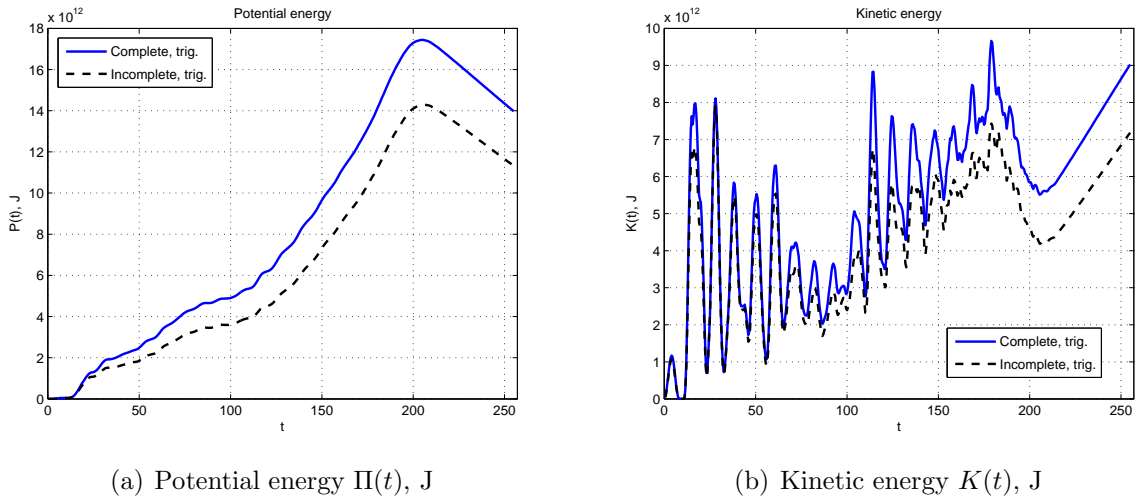
FIGURE 10. Energy evolution during our simulations in the complete (blue solid line) and incomplete (black dotted line) scenarios using the finite fault inversion by Caltech Tectonics Observatory [Ozg06]. Note that the scales are different on the left and right images. The time t is given in seconds.
