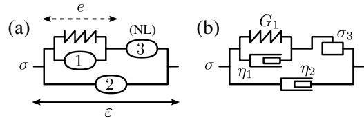
FIG. 1: Schematic, scalar view of rheological models (deformation \varepsilon and stress \sigma ) with only one internal degree of freedom, namely the deformation e of the spring. (a) General model: it has one (non-linear) spring and three creeping elements, each of which may have a flow threshold. (b) Foams and emulsions display some (large) deformation before creep is triggered. Hence, creep elements 1 and 2 cannot have a finite threshold. By contrast, element 3 does have a threshold. Here, for simplicity, we assume that the spring and both viscous elements are linear, and that element 3 cannot withstand any stress beyond \sigma_3 .
