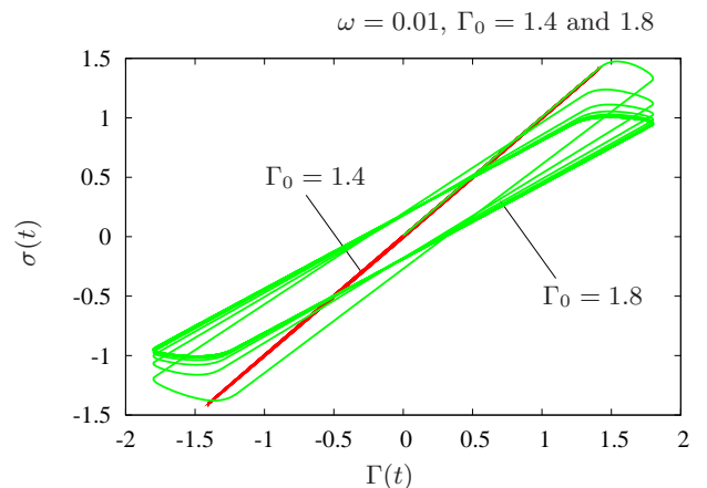
FIG. 6: Large amplitude oscillatory simulations: shape of \sigma_{xy}(t) versus \Gamma(t) (Lissajous) curves, obtained for a = b = 1/7 , \omega = 0.01 , \Psi = 0.1 and \mathcal{K} = 1 . Top: transition from elastic to plastic behaviour as the amplitude is increased. At very large amplitudes, an overshoot is apparent like in continuous shear situations. Bottom: in a slightly plastic situation (amplitude 1.8), it takes several cycles before the system behaves in a periodic manner.
