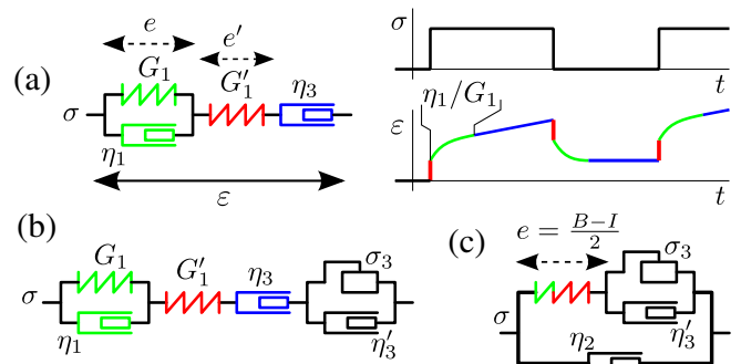
FIG. 3: (a) Burger model: schematic diagramme (left) and deformation response \varepsilon(t) to a step imposed stress \sigma(t) . Spring G'_1 elongates immediately (red segment) while spring G_1 responds with some delay (green curve) due to viscous element \eta_1 . Viscous element \eta_3 gives rise to a constant additional deformation rate (blue segment). (b) Combined Bingham-Burger model: solid friction element \sigma_3 (complemented by viscous element \eta'_3 ) is now included so as to provide additional creep above the stress threshold. We believe that some tensorial version of this model could mimic the rheological behaviour of a foam quite adequately. (c) Model studied in the present work. Apart from the additional viscosity \eta_2 introduced in Fig. 1, it represents the combined Bingham-Burger model when the (blue) viscous element has not been deformed yet, either at intermediate time scales when the (green) Voigt element has relaxed (the green and red springs then respond in series) or at short time scales when the Voigt element is still blocked (in which case only the red spring responds).
