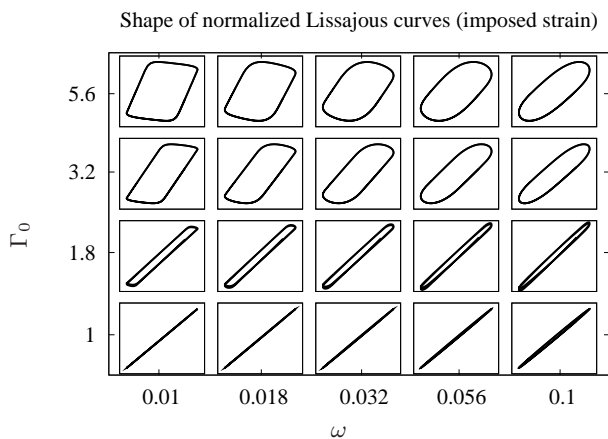
FIG. 5: Large amplitude oscillatory simulations: shape of \Gamma(t) versus \sigma_{xy}(t) (Lissajous) curves, obtained for a = b = 1/7 , \Psi = 0.1 and \mathcal{K} = 1 . Top: range from \omega = 0.01 to \omega = 100 and \Gamma_0 = 0.1 to \Gamma_0 = 100 . Bottom: zoom on a more restricted range of parameters.
