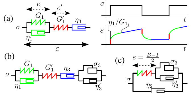
FIG. 3: (a) Burger model: schematic diagramme (left) and deformation response \varepsilon(t) to a step imposed stress \sigma(t) . Spring G_1' elongates immediately (red segment) while spring G_1 responds with some delay (green curve) due to viscous element \eta_1 . Viscous element \eta_3 gives rise to a constant additional deformation rate (blue segment). (b) Combined Bingham-Burger model: solid friction element \sigma_3 (complemented by viscous element \eta_3' ) is now included so as to provide additional creep above the stress threshold. We believe that some tensorial version of this model could mimic the rheological behaviour of a foam quite adequately. (c) Model studied in the present work. Apart from the additional viscosity \eta_2 introduced in Fig. 1, it represents the combined Bingham-Burger model when the (blue) viscous element has not been deformed yet, either at intermediate time scales when the (green) Voigt element has relaxed (the green and red springs then respond in series) or at short time scales when the Voigt element is still blocked (in which case only the red spring responds).
