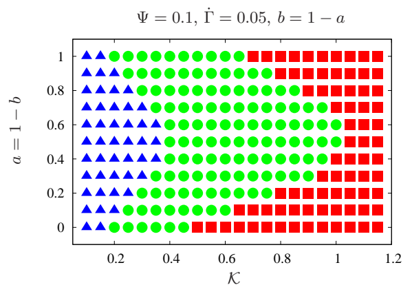
FIG. 14: Comparison of 0D and 1D simulations in plane (\mathcal{K}, a) , using b = 1 - a , \dot{\Gamma} = 0.05 and \Psi = 0.1 . Blue triangles indicate values for which the 0D model allows only uniform flow. Red squares indicate values for which shear banding was obtained in the 1D simulation for the initial conditions chosen. Green disks indicate additional values for which the 0D model allows shear banding.
