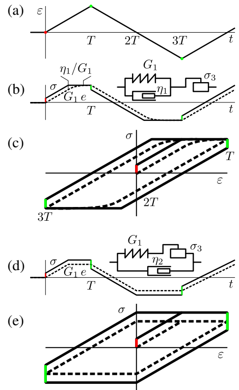
FIG. 2: Response of the model represented in Fig. 1b to a triangle wave deformation. (a) Deformation \varepsilon as a function of time. (b) In the limit \eta_2 = 0 , stress \sigma (solid line) and elastic stress G_1 e transmitted by the spring (dashed line) as a function of time. When the threshold \sigma_3 is reached, the spring relaxes with the time scale \eta_1/G_1 of the Voigt element. (c) Corresponding Lissajous representation of \sigma and G_1 e . The periodic jump in stress (green segment) has the same amplitude as the initial jump (red segment). (d) In the limit \eta_1 = 0 , stress \sigma (solid line) and elastic stress G_1 e transmitted by the spring (dashed line) as a function of time. (e) Corresponding Lissajous representation of \sigma and G_1 e . The amplitude of the periodic jump in stress (green segment) is twice that of the initial jump (red segment).
