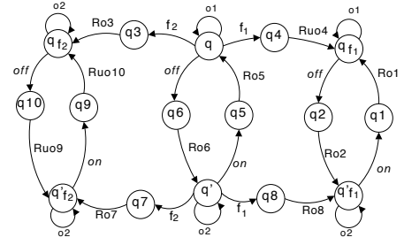
Figure 5. The behavior automaton
