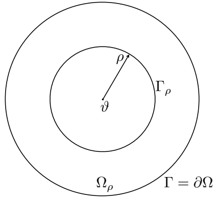
Fig. 1 The domain \Omega_\rho in two spatial dimensions.
