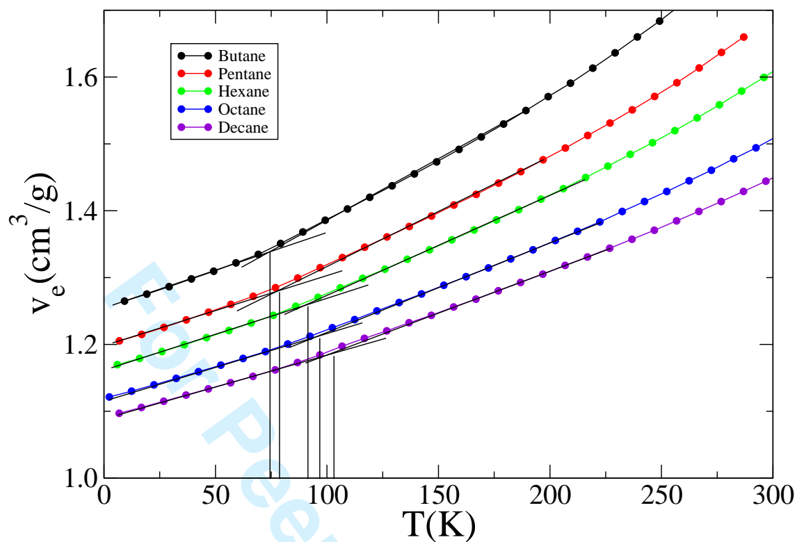
FIG. 2: Plot of the specific volume as a function of the temperature for butane (black filled circles), pentane (red filled circles), hexane (green filled circles), octane (blue filled circles) and decane (violet filled circles). The glass transition is estimated by the crossing of the best-fitted to the data straight thin lines below and above the glass transition.
