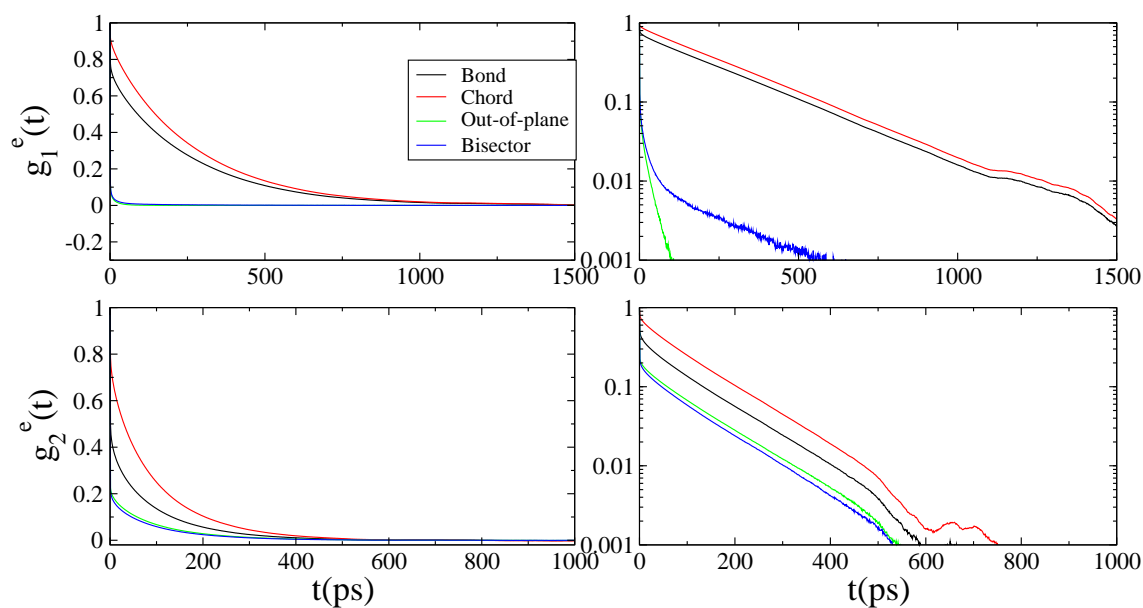
FIG. 8: Orientational autocorrelation functions g_1^e(t) (upper row) and g_2^e(t) (lower row) for the pentane at T = 96.92 K. The left panels correspond to a linear scale, and the right panels are the same plot in log-lin scale.
