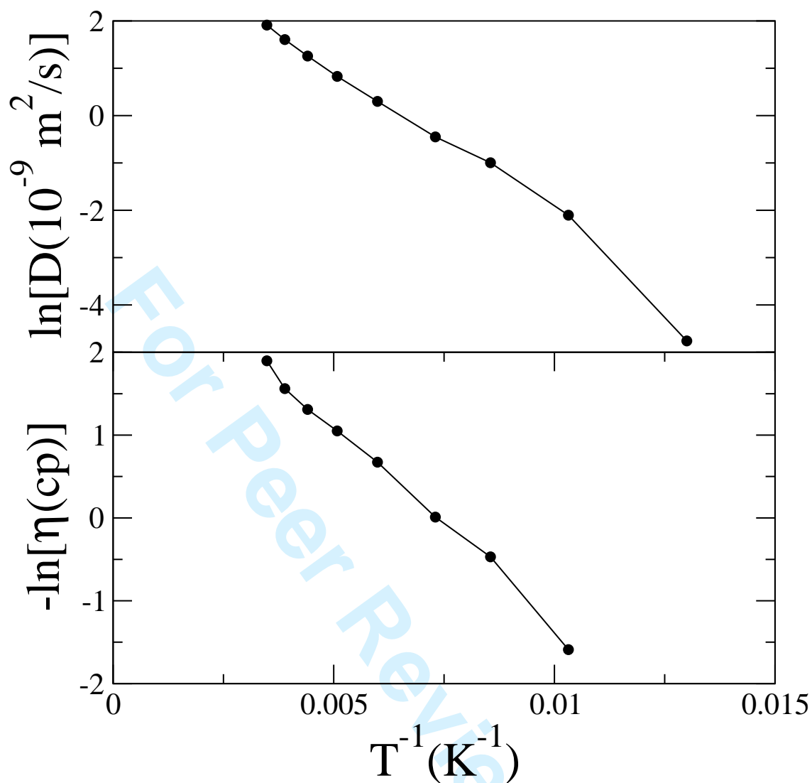
FIG. 6: Upper panel: Arrhenius plot of the self-diffusion coefficient D for the pentane. Lower panel: Arrhenius plot of the pentane shear viscosity \eta . Lines are drawn through as a guide to the eye.
