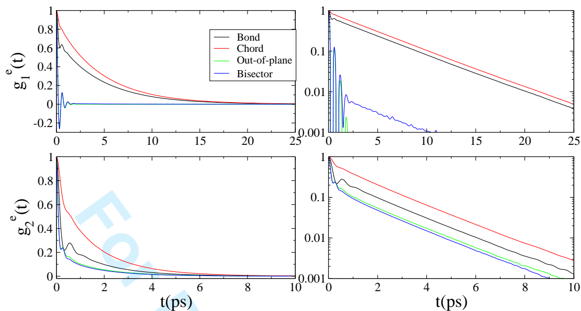
FIG. 7: Orientational autocorrelation functions g_1^e(t) (upper row) and g_2^e(t) (lower row) for the pentane at T = 286.92 K. The left panels correspond to a linear scale, and the right panels are the same plot in log-lin scale.
