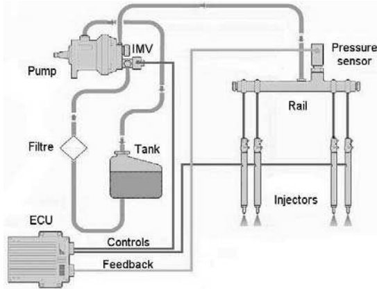
Figure 2 : Common rail diesel injection system
