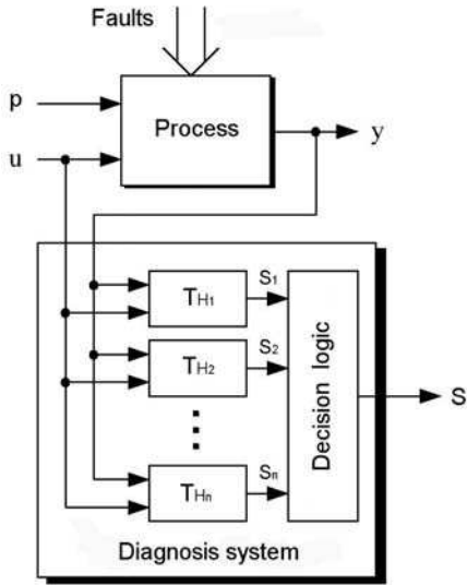
Figure 1 : Structured hypothesis tests based diagnosis system
