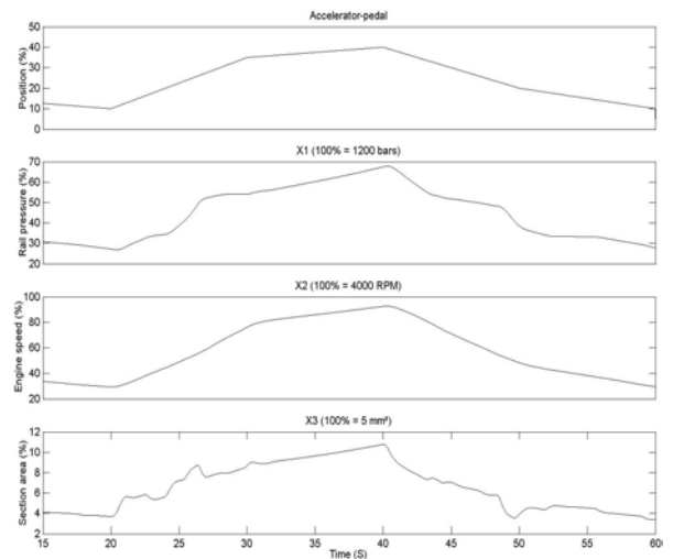
Figure 3 : Fault-free pressure control process simulation
