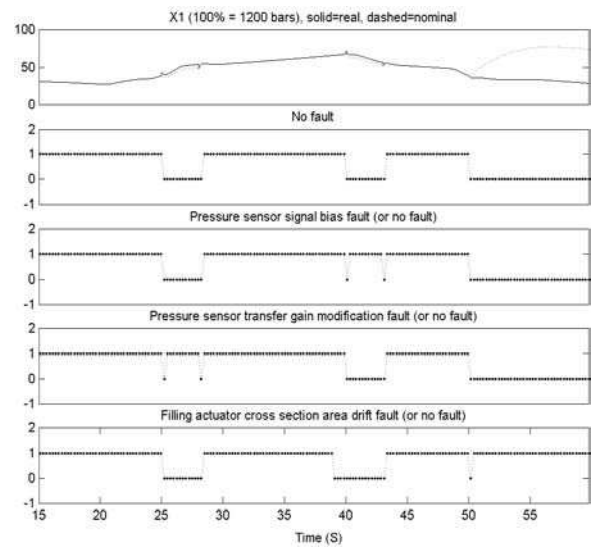
Figure 4 : Results of hypothesis tests applied to a faulty pressure control loop
