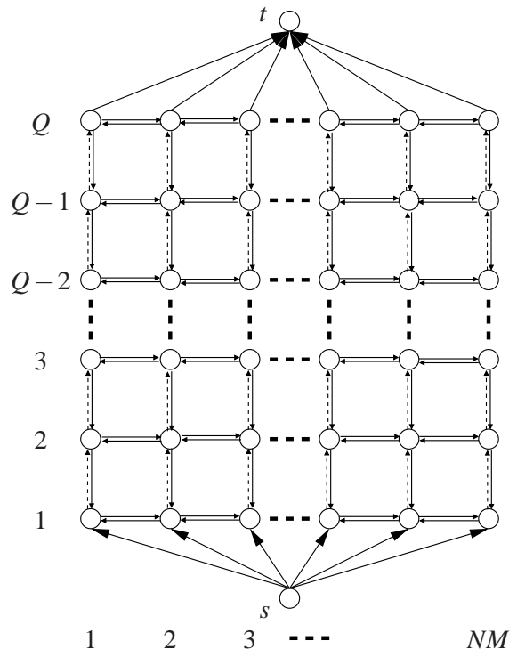
Fig. 1 Construction of the Ishikawa-like optimization graph. Arrows represent the edges \mathcal{E} and circles the nodes in \mathcal{V} . Horizontal edges are in \mathcal{E}_{\mathcal{P}} , the dotted upward vertical edges are in \mathcal{E}_{\mathcal{D}} and the plain downward vertical edges are in \mathcal{E}_{\mathcal{C}} . Vertices s and t are respectively the source and the sink. All pixels in the image from 1 to NM are represented in the columns. In actual 2D images, there exist many more penalty edges \mathcal{E}_{\mathcal{P}} than depicted here: all those between neighbours in \mathbb{V} .
