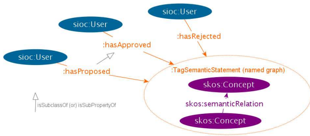
Figure 1: SRTag RDF schema
