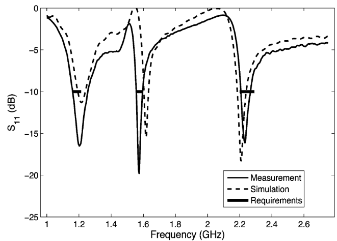
Fig. 4: S_{11} of the pyramidal GPS/GALILEO/MicroSat triband antenna [1].
