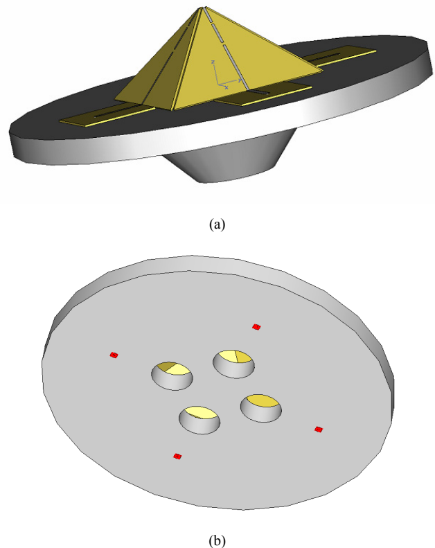
Fig. 6: Ground plane configurations [4]: (a) Ground plane loaded with truncated conical cut-off open-ended waveguide; (b) Ground plane with multiple holes.
