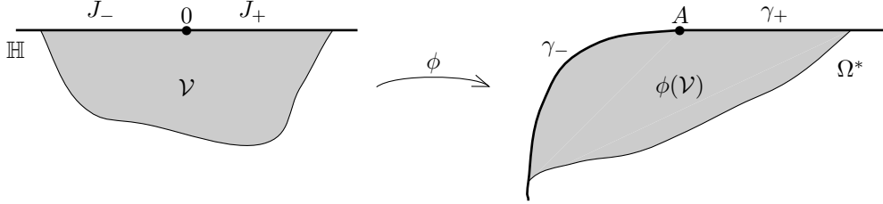
Figure 2: Conformal parametrization
