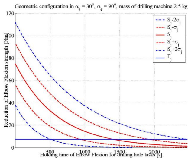
Figure 6: Reduction of the elbow strength while holding a drilling machine weighted as 2.5 kg
