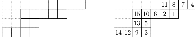
Fig. 4: The skew shape corresponding to the underlying unlabelled poset of Figure 1, and the skew Young tableau corresponding to the permutation \sigma of Figure 1.
