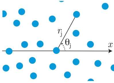
FIG. 13: An infinite 3D medium with spherical scatterers is considered. The position of scatterer 0 is arbitrarily chosen as the centre of the coordinates and we look for modes of the system consisting of plane waves propagating in the x direction. The dispersion relation is obtained by calculating the total field experienced by scatterer 0 due to the other scatterers.
