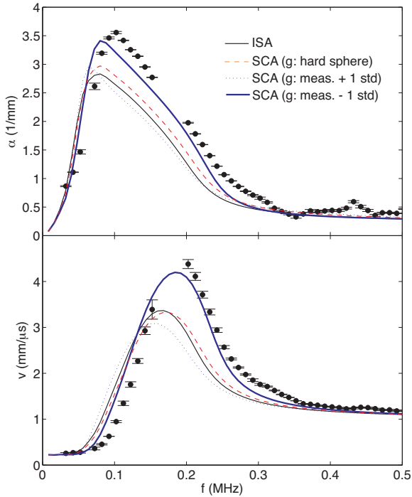
FIG. 12: The effect of polydisperse correlations as predicted by the self-consistent approach (SCA). Three g(R, r) functions are considered (see figure 11): hard-sphere correlation (dashed lines), high and low estimates of g measured from the x-ray data (dotted and thick lines, respectively).
