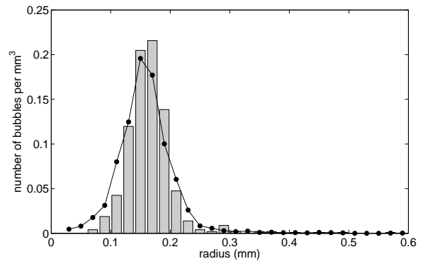
FIG. 3: Histogram of the bubble radius distribution for the sample in figure 2, obtained from the image analysis. The superposed curve (circles plus connecting lines) corresponds to the result of the x-ray tomography analysis.
