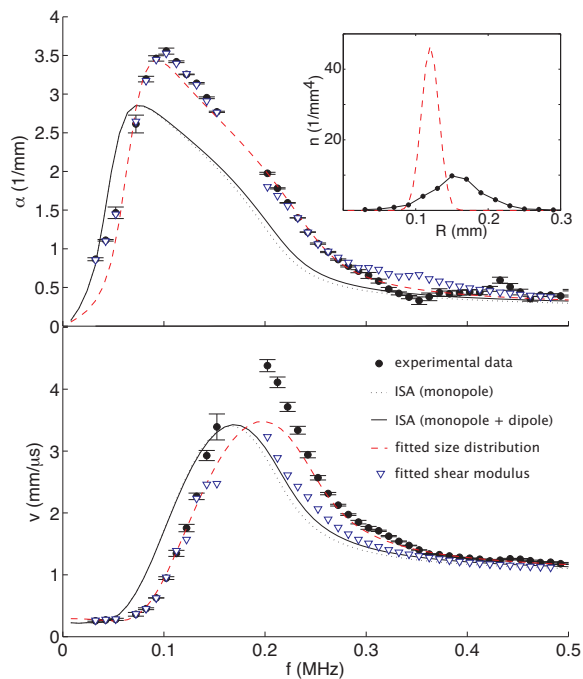
FIG. 5: Close-up of the attenuation and velocity peaks. Solid circles correspond to experimental data (same as in Fig. 4). Comparison with Foldy’s model is shown for monopolar scattering of the bubbles (dotted lines) and monopolar + dipolar scattering (solid lines). Note that there are no adjustable parameters in this comparison of the theory with experiment. Results of fitting the model to the data by allowing either the size distribution (dashed lines) or the shear modulus (triangles) to vary are also shown. In the inset, the size distribution determined by the x-ray experiment (solid line) is compared to the one inferred from the fit to the ultrasonic data (dashed lines).
