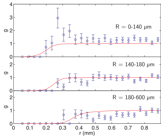
FIG. 11: Function g(r, R) as measured from the x-ray tomography data (circles) on three populations of bubble radii. Error-bars correspond to one standard deviation. The solid line corresponds to the hard-sphere approximation for the bubble size distribution measured in the sample.
