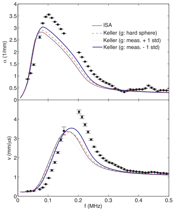
FIG. 10: Investigation of the effect of correlations. The experimental attenuation and velocity (circles) and the ISA prediction (solid thin lines) are shown again, as in figure 4. Keller's approach (Eq. (14)) is plotted for the hard-sphere correlation (dashed lines), for the high estimation of g measured from the x-ray data (dotted lines), and for the low estimation of g (thick solid lines).
