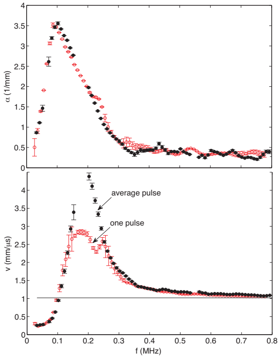
FIG. 4: Attenuation and phase velocity in the bubbly PDMS sample, measured from a single pulse (open circles) and from an average pulse (solid circles). The velocity in the pure PDMS is shown by the solid line. The attenuation in pure PDMS is, on average, 2 orders of magnitude less than in the bubbly sample (too small to be visible on the graph).
