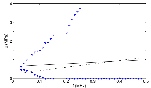
FIG. 6: Shear moduli as functions of frequency. The lines correspond to the results for experimental \mu' (solid line) and \mu'' (dashed line), as given in equations (12). Open triangles show the fitted values for \mu' , solid ones for \mu'' .
