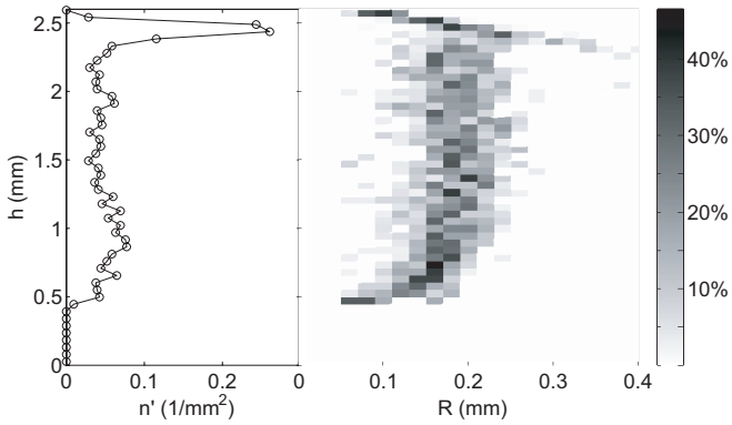
FIG. 7: The layered structure of the sample is revealed by the x-ray tomography. Along the thickness h of the sample, we report the number of bubbles per unit area n' (left) and the radii distribution histogram (right) for each layer.
