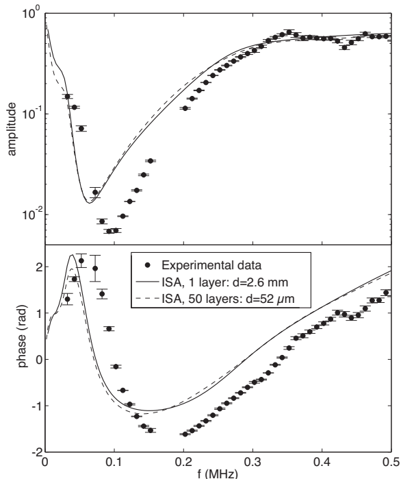
FIG. 8: Amplitude (top) and phase (bottom) of the acoustic transmission through the sample. Because the data are the same as in figure 5, the same discrepancy between Foldy's prediction for a homogenous sample (solid lines) and the experimental data (circles) is obtained. The prediction for a layered medium (dashed lines) does not bring better agreement.
