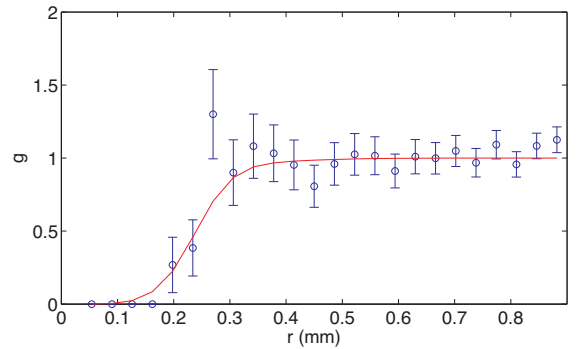
FIG. 9: Function g as measured from the x-ray tomography data (circles). Error-bars correspond to one standard deviation. The solid line corresponds to the hard-sphere approximation for the bubble size distribution measured in the sample.
