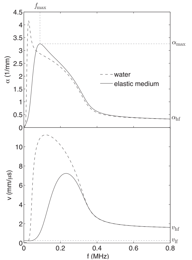
FIG. 1: Predictions of the ISA for the attenuation (top) and phase velocity (bottom) as functions of frequency for bubbles in water (dashed lines) and in an elastic matrix (solid lines) with \mu' = 0.7 \text{ MPa} , \mu'' = 0.4 \text{ MPa} ; the bubble concentration is 2% and the mean radius is taken to be 150 \mu\text{m} with a 25% polydispersity. The characteristic features ( f_{\text{max}} , \alpha_{\text{max}} , \alpha_{\text{hf}} , v_{\text{lf}} , and v_{\text{hf}} ) are indicated.
