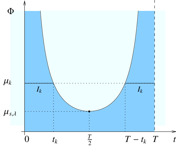
Figure 1: The function \Phi . The shaded region is treated in the first step of the proof.
