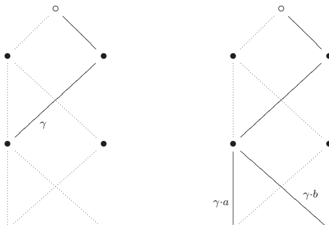
Figure 2: Example of eigenvectors of \Delta_s for the Fibonacci diagram.
