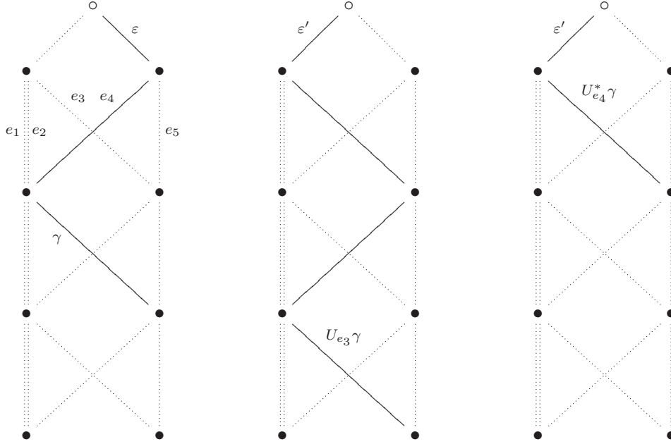
Figure 4: Example of some Cuntz–Krieger operators acting on finite paths.
