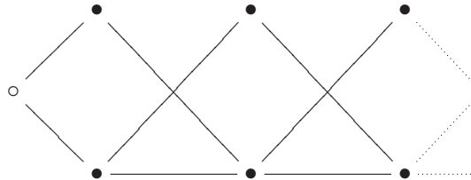
Figure 1: A self-similar Bratteli diagram associated with the matrix \begin{pmatrix} 1 & 1 \\ 1 & 0 \end{pmatrix} (root on the left).
