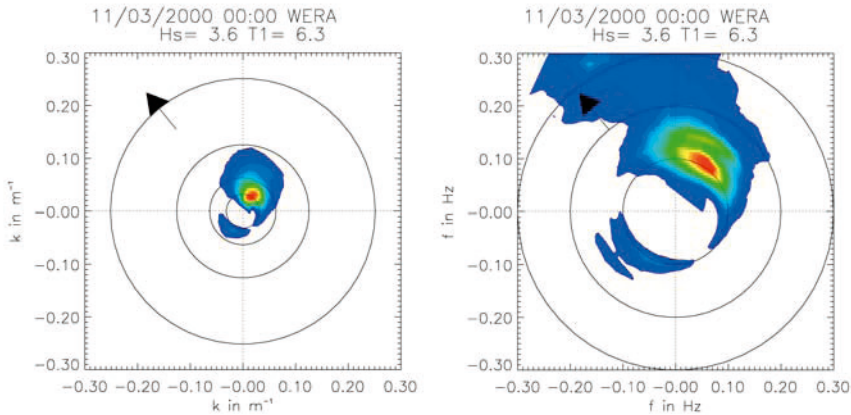
Figure 5.16: Directional spectra measured by the HF radar WERA at the Norwegian coast ( H_s in metres and T1 = Tm01 in seconds). To the left is shown the wavenumber spectrum with circles shown at wavelengths of 200 m, 100 m, 50 m and 25 m. The directional frequency spectrum is shown to the right. The arrows show radar measured wind direction. The spectral peak is at a wavelength of about 200 m and period of about 9 second propagating towards the north-west. Winds are offshore, generating waves at higher frequencies in the wind direction as can be seen in the frequency spectrum. The colour coding is 20 equally spaced intervals from 0 to the maximum. The windwave peak has an amplitude about 20 percent of the maximum.
