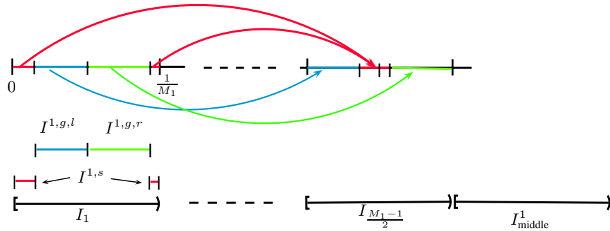
Fig. 5. \tau_2 for the ‘‘singular’’ indices on the left side.
