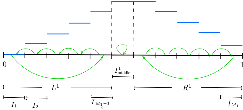
Fig. 1. Representations of \varphi^1 and \tau^1 .
