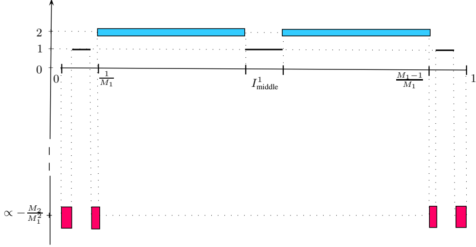
Fig. 3. Shape of the quasi-cost \varphi^2 + \psi^2 \circ T_{\alpha_2}^{(\tau_2)} .
