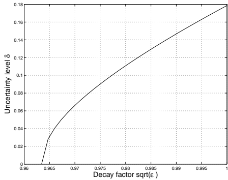
Fig. 2. Tradeoff performance/robustness
