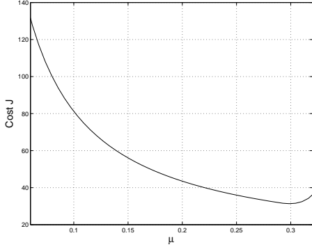
Fig. 1. Line search \mu
