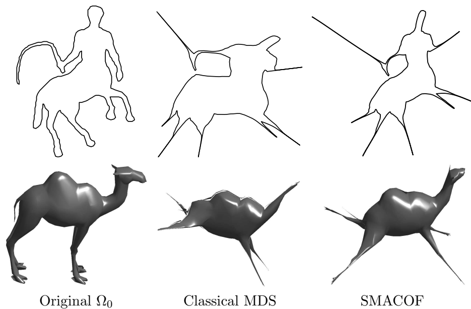
Fig. 5.3 Examples of bending invariance computed using classical MDS and SMACOF, 2D shape (top row) and for a 3D surface (bottom row).
