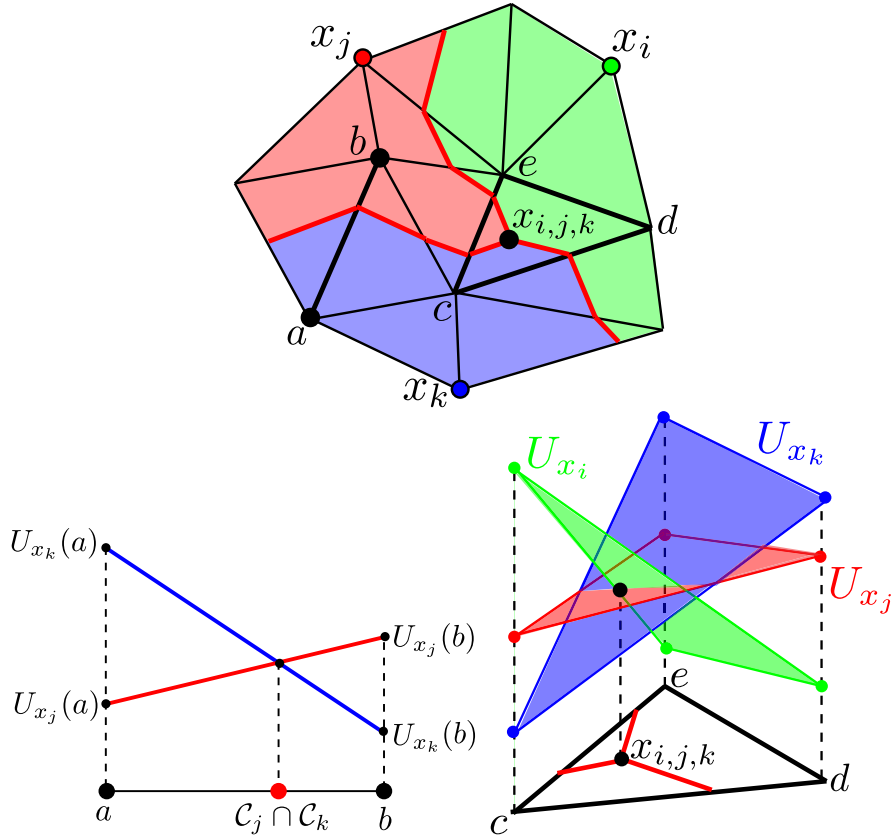
Fig. 2.16 Top: extraction of piecewise affine Voronoi boundaries on 2D triangulations. Bottom: the geodesic distances on the edge (a, b) and triangle (c, d, e) extracted from the triangulation on the top are displayed as affine functions.
